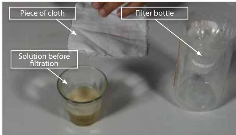
V. Take a bottle and cut off the top part and turn it over into the bottle. Place a piece of cloth into the cone-like shape.
