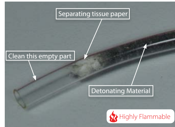
VI. Fill the open end with a peice of tissue paper. Wipe the inner tip so that it doesn't burn when sealed with the heat sealer.
