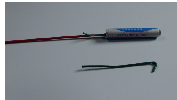
5. Remove the fuse from the firework.
